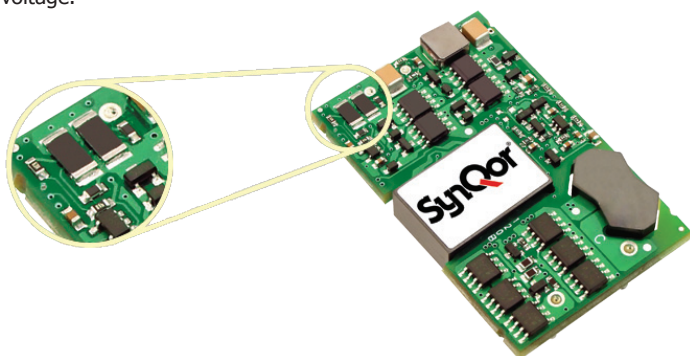
Figure G: Location of Sense Resistor
