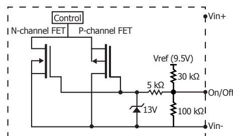
Figure B: Internal ON/OFF pin circuitry
