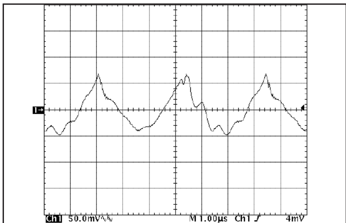
Figure 15: Output voltage ripple at nominal input voltage and rated load current (50 mV/div). Load capacitance: 1\ \mu\text{F} ceramic capacitor and 15\ \mu\text{F} tantalum capacitor. Bandwidth: 20 MHz. See Figure 12.
