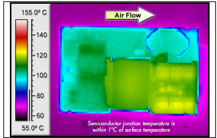
Figure 8: Thermal plot of converter at 25 A load current (300 W) with 55 °C air flowing at the rate of 200 LFM. Air is flowing across the converter from input to output (nominal input voltage).
