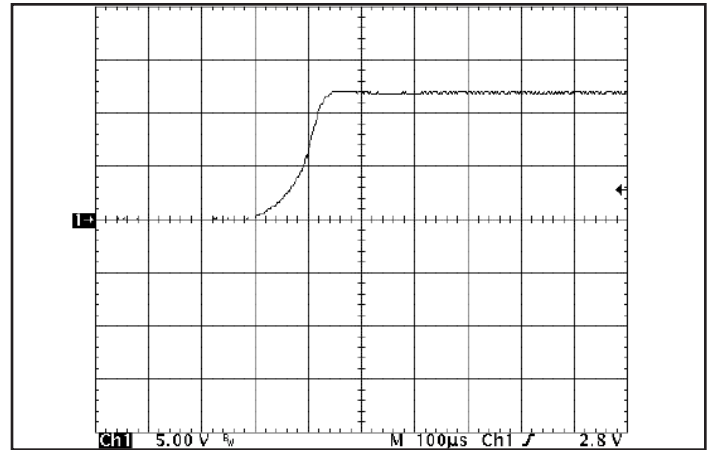
Figure 10: Turn-on transient at zero load (100 μs/div). Ch 1: V_{out} (5 V/div)
