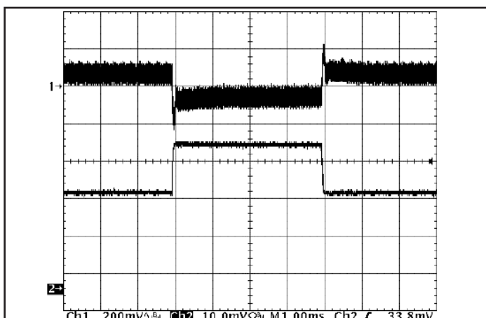
Figure 11: Output voltage response to step-change in load current (50%-75%-50% of I_{out(max)} ; dI/dt = 0.1 A/μs). Load cap: 15 μF, 100 mΩ ESR tantalum cap and 1 μF ceramic cap. Top trace: V_{out} (200 mV/div), Bottom trace: I_{out} (5 A/div).
