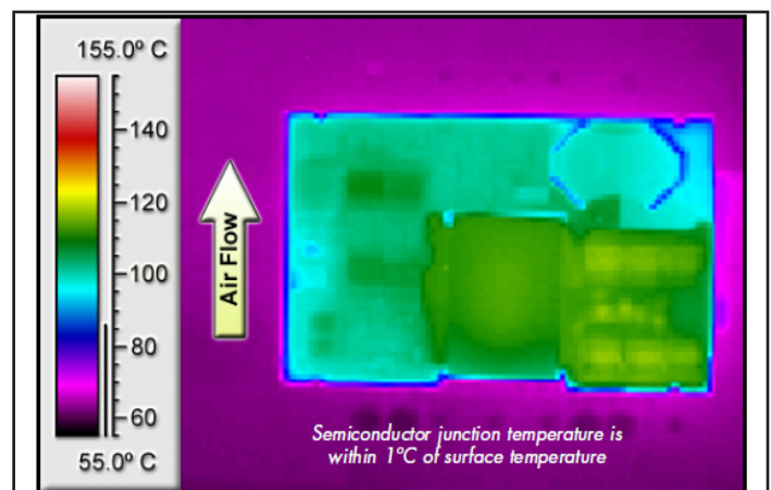
Figure 6: Thermal plot of converter at 25 A load current (300 W) with 55 °C air flowing at the rate of 200 LFM. Air is flowing across the converter from pin 3 to pin 1 (nominal input voltage).
