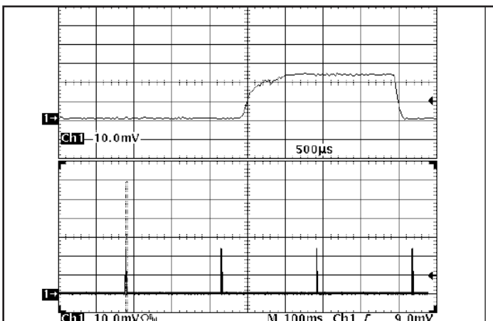
Figure 17: Load current ( 50\ \text{A/div} ) as a function of time when the converter attempts to turn on into a 1\ \text{m}\Omega short circuit. Top trace ( 500\ \mu\text{s/div} ) is an expansion of the on-time portion of the bottom trace.
