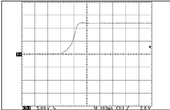
Figure 9: Turn-on transient at full load (resistive load) (100 μs/div). Ch 1: V_{out} (5 V/div)
