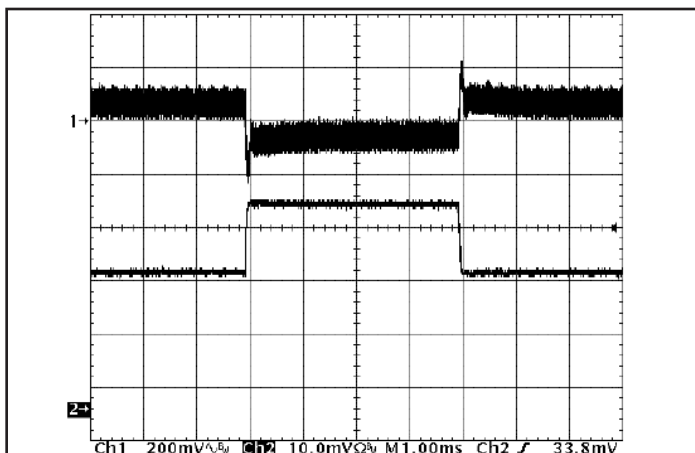
Figure 11: Output voltage response to step-change in load current (50%-75%-50% of I_{out(max)} ; dI/dt = 0.1 A/\mu s ). Load cap: 15 μF, 100 mΩ ESR tantalum cap and 1 μF ceramic cap. Top trace: V_{out} (200 mV/div), Bottom trace: I_{out} (5 A/div).
