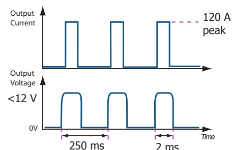
Figure D: Output Short Circuit and Auto-Resetting protection diagram (not to scale)
