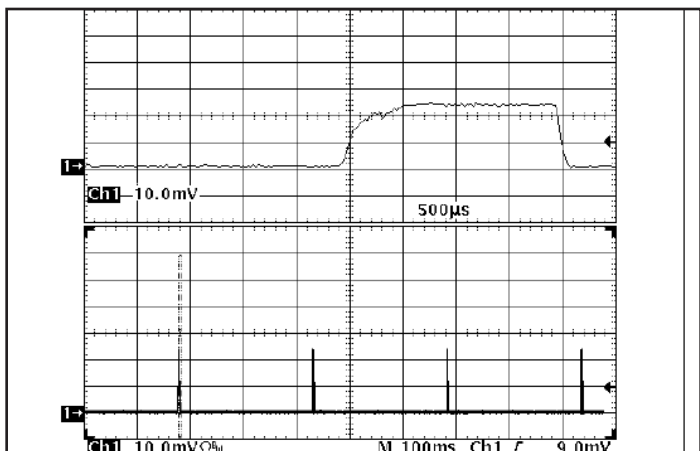
Figure 17: Load current (50 A/div) as a function of time when the converter attempts to turn on into a 1\ \text{m}\Omega short circuit. Top trace ( 500\ \mu\text{s}/\text{div} ) is an expansion of the on-time portion of the bottom trace.
